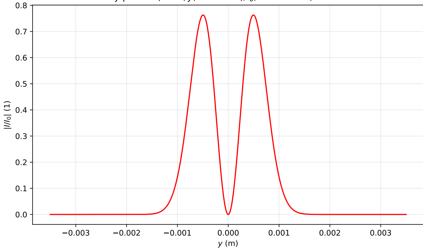
Intensity profile I(x=0, y, z=0.080)/I_0 , P_{in}=0.5P_{cr} , artificial time
